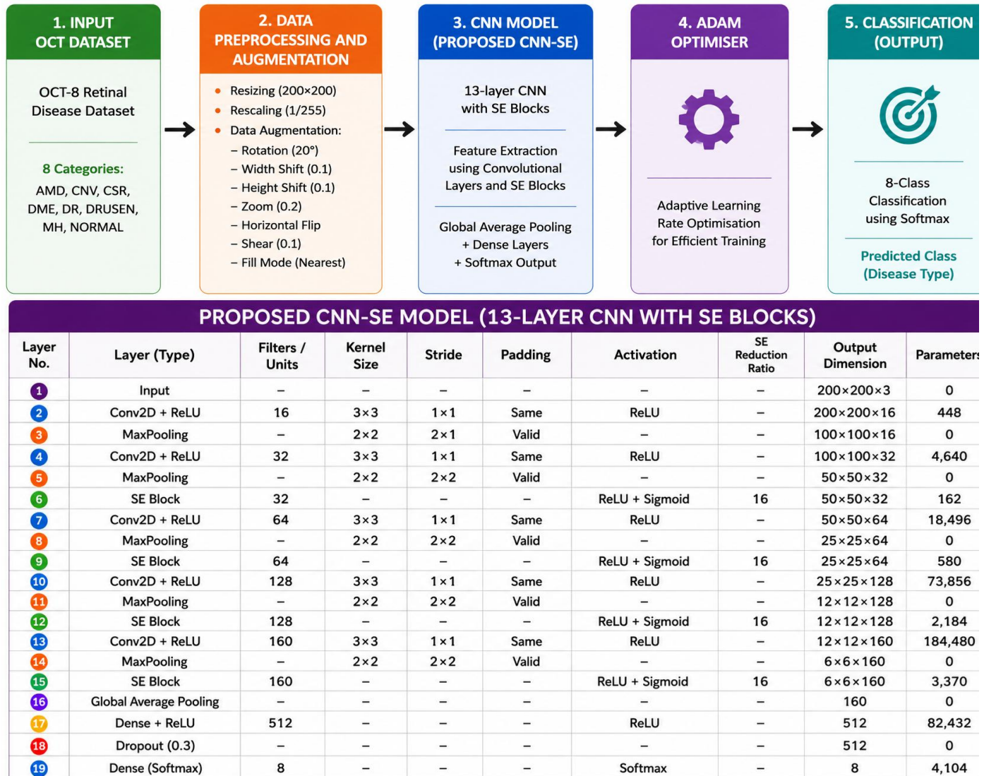
Fig. 1. Proposed CNN Model (OCT-C8: 8 Class, OCT2017: 4 Class)
