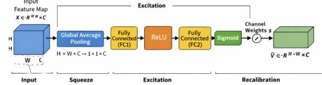
Fig. 2. Architecture of SE block
